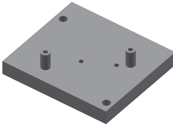
Figure 1: Jig for drilling 0.063 inch hole Own design
